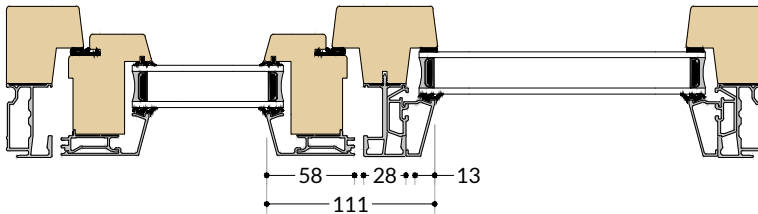
B-B Mullion for fixed sidelight
