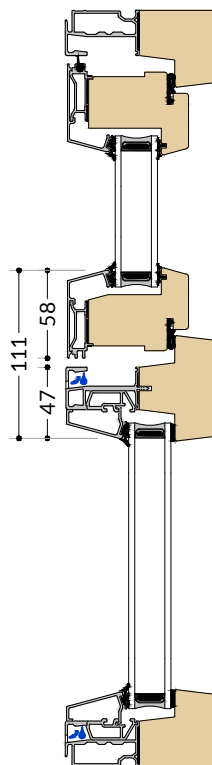
B-B Mullion for fixed sidelight
