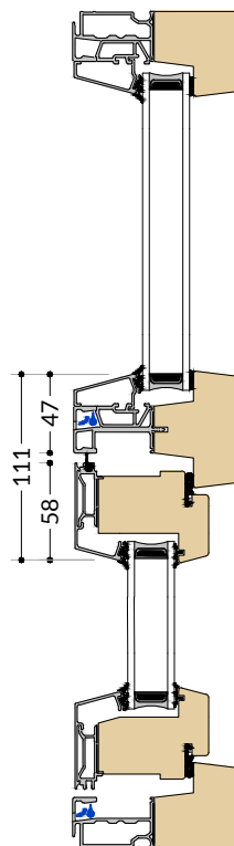
E-E Transom for fixed upper light
