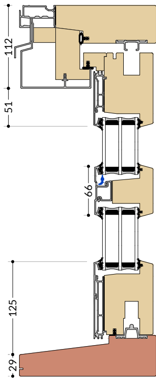
B-B SDA Sliding Leaf Midrail
