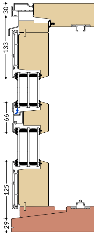
C-C SDA Fixed Leaf Midrail
