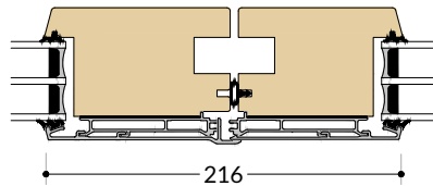
E-E SDC Meeting Stile
