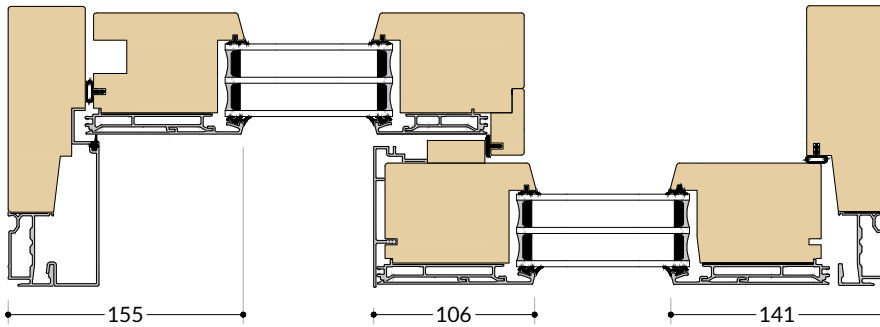
A-A SDA Mullion
