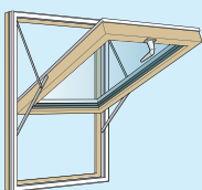
TSG 180 Fully Reversible 180° Opening
